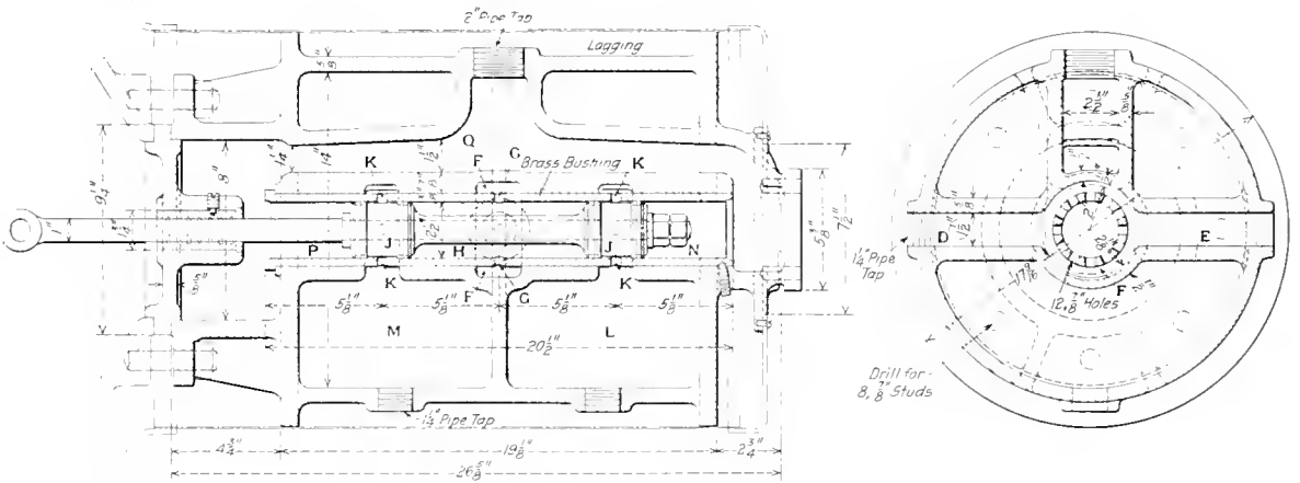
Details of the Vincent Drifting Valve for the D. & R. G. Locomotives
